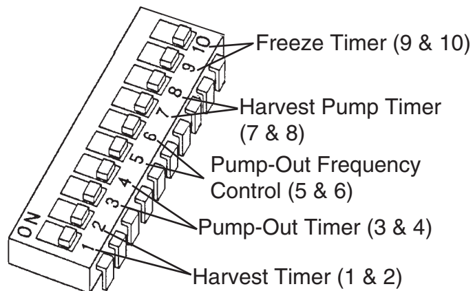
S1 Dip Switch
