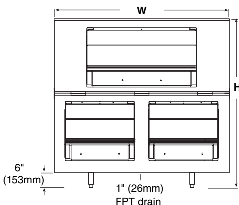
Front View - Double Section Bin
