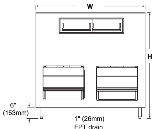
Front View - Single Section Bin
